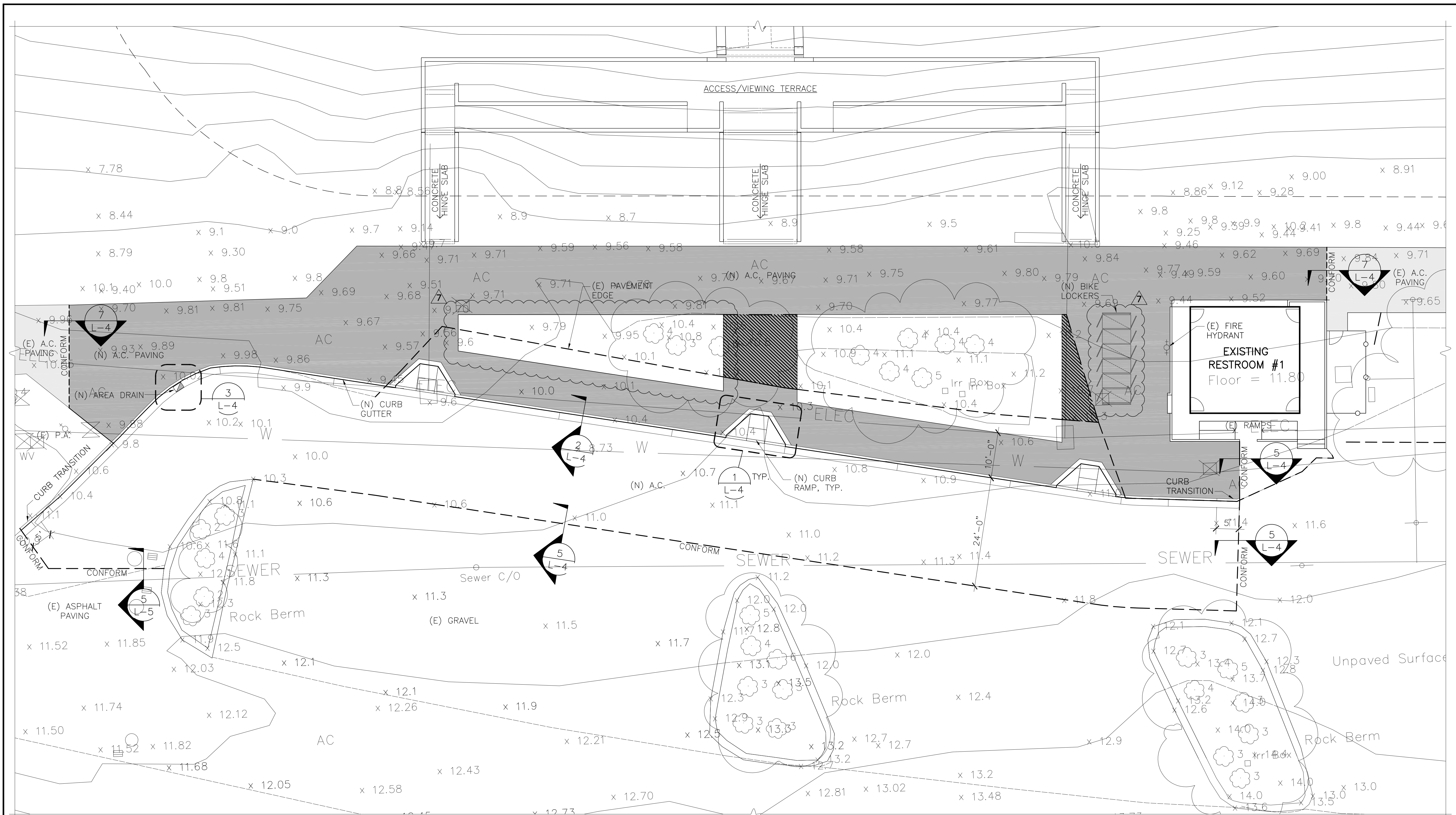
1 SITE IMPROVEMENTS AND PAVING PLAN SCALE: 1" = 10'
